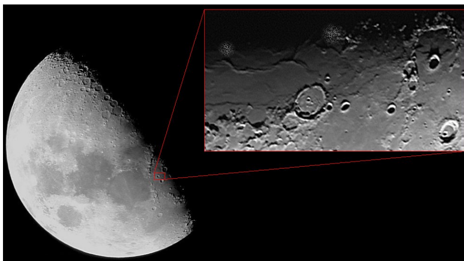
Photograph of Apogee (left smudge) and Perigee (right smudge)
